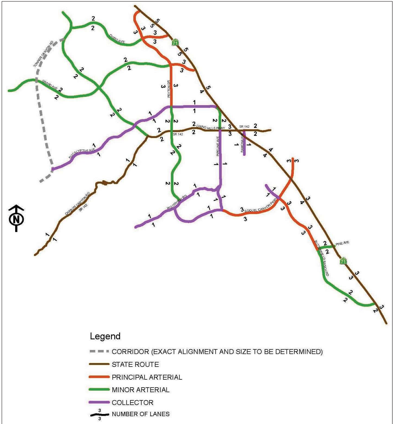
Figure 2-1 – Roadway Plan
